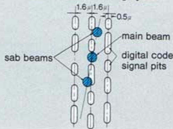
3-beam laser tracking system
